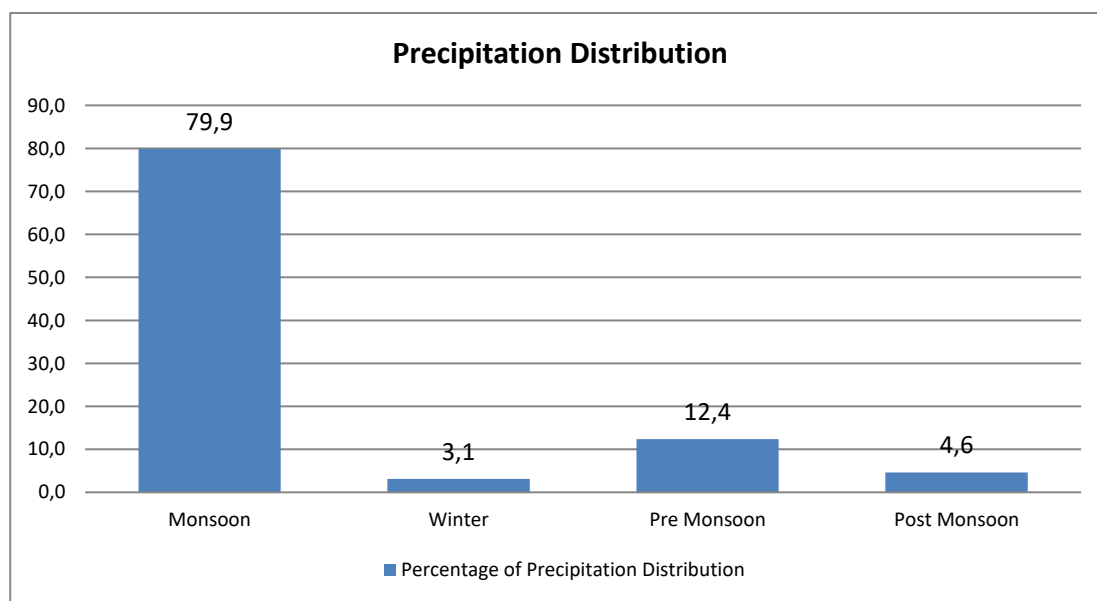
Figure 1. Precipitation Distribution
