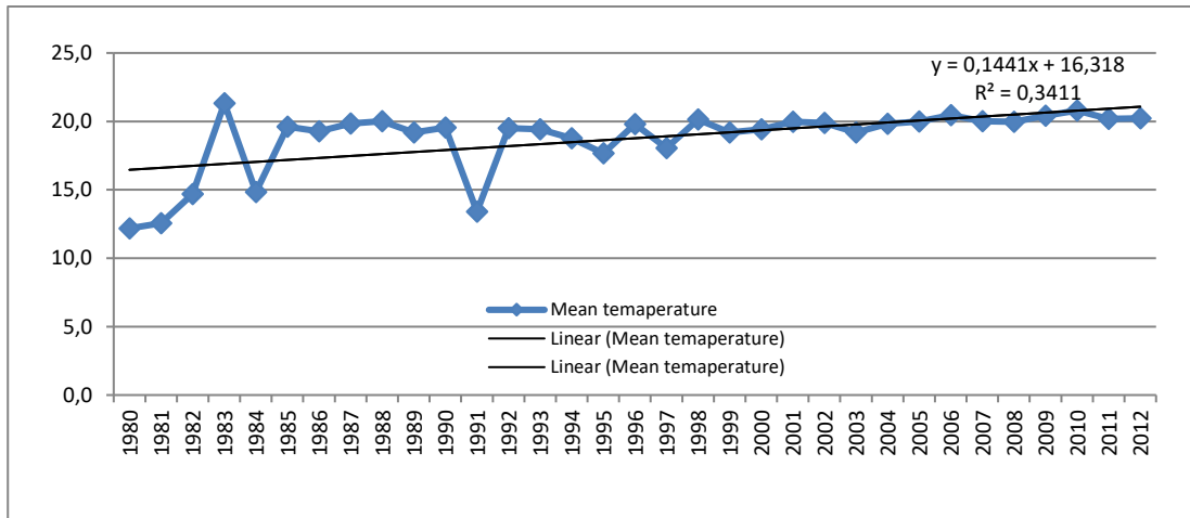
Figure 2. Mean Temperature
